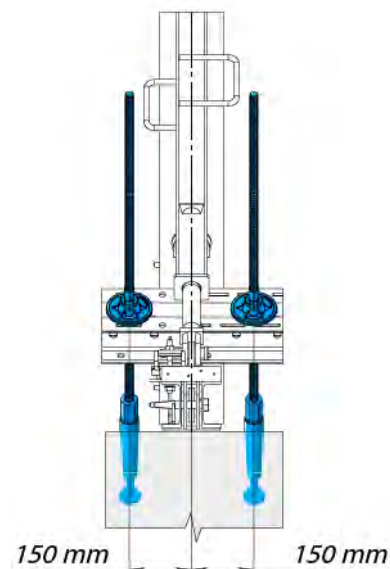
Distance between anchors for either pigtail anchor or stop-anchor system.
