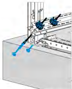
Anchoring with a stop-anchor
